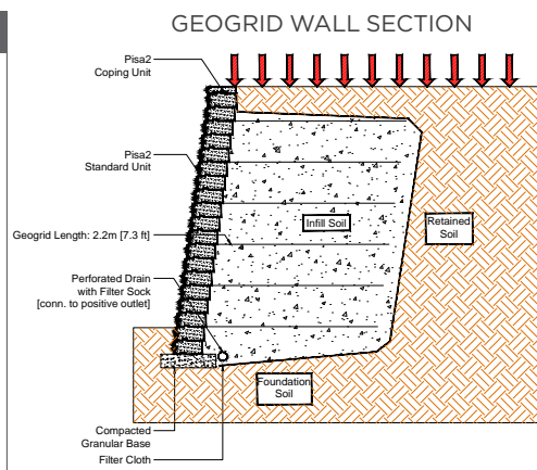
Cross sections are examples, and must not be used for construction.
