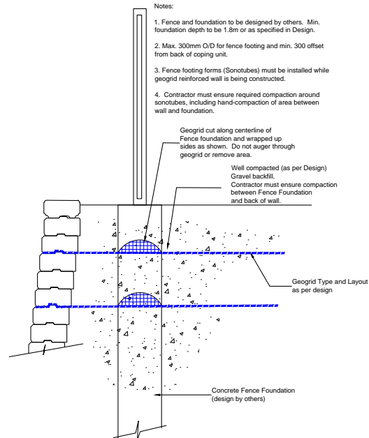
TYPICAL DETAIL PRIVACY FENCE
